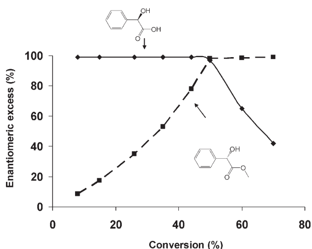
Figure 4. Evolution of enantiomeric excess ( ee ) of 1 and 3 versus hydrolysis conversion of ( \pm )- 1 catalyzed by aminated BrCN-CAL-B immobilized preparation. Experiments were performed using 10 mM of substrate at pH 7 and 4 °C. ee of [( R )- 1 ] (square), ee of released acid [( R )- 3 ] (rhombus).
