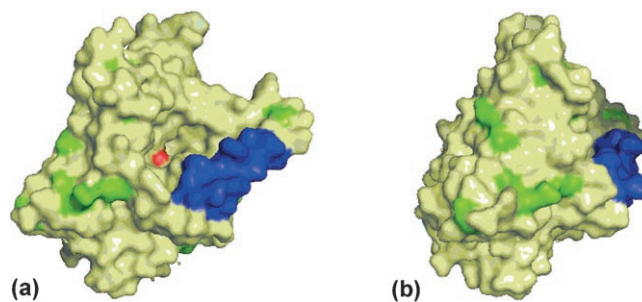
Figure 3. 3D surface model structure of PFL. a) lid face, b) lateral face. Asp or Glu residues (green), lid oligopeptide (blue), catalytic serine (red). The 3D structure was obtained from the Protein Data Bank (PDB) using Pymol vs. 0.99. The pdb code for PFL is 2LIP.
