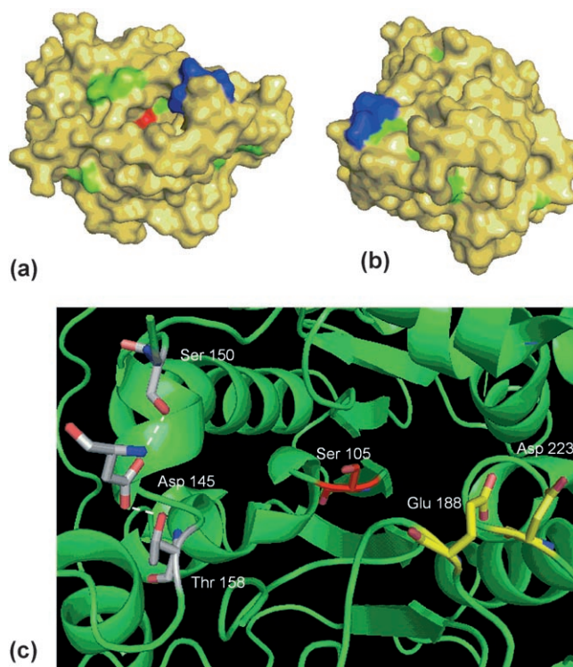
Figure 1. 3D surface model structure of CAL-B. a) lid face, b) lateral face. Asp or Glu residues (green), lid oligopeptide (blue), catalytic serine (red); c) Representation of the active site surrounded of the CAL-B marking the key amino acid. The 3D structure was obtained from the Protein Data Bank (PDB) using Pymol vs. 0.99. The pdb code for CAL-B is TCA.
