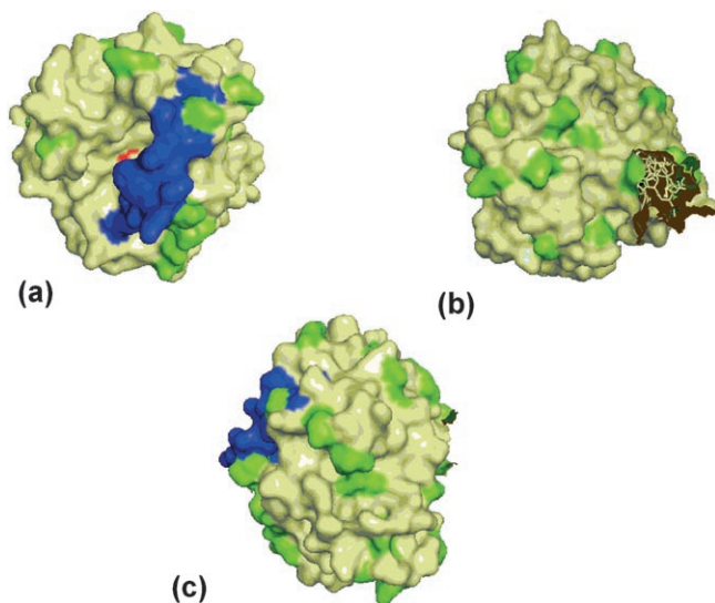
Figure 2. 3D surface model structure of TLL. a) lid face, b) lid opposite face c) lateral face. Asp or Glu residues (green), lid oligopeptide (blue), catalytic serine (red). The 3D structure was obtained from the Protein Data Bank (PDB) using Pymol vs. 0.99. The pdb code for TLL is 1DTB.
