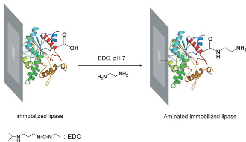
Scheme 4. Chemical amination of protein carboxyl groups. EDC=1-ethyl-3-(3-dimethylaminopropyl)carbodiimide hydrochloride.
