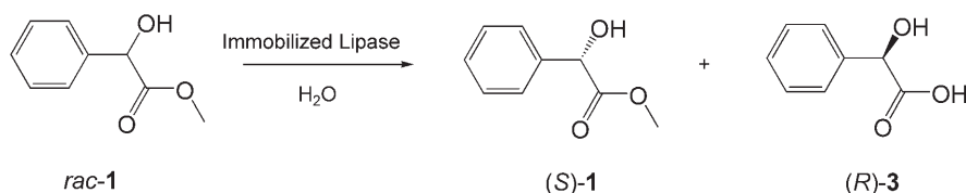
Scheme 2. Enzymatic kinetic resolution of ( \pm )- 1 .
