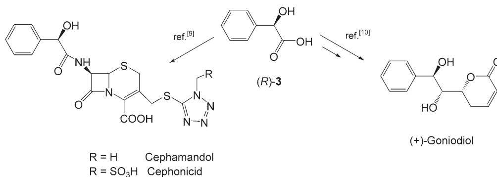
Scheme 1. Synthesis of biologically active compounds from ( R )-mandelic acid.
