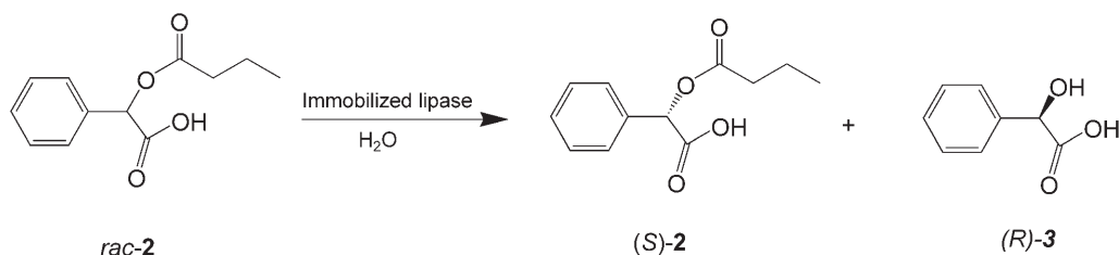
Scheme 3. Enzymatic kinetic resolution of (±)-2.
